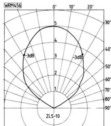
Fig. 4.3: Horizontal radiation pattern of the ZL5-10
