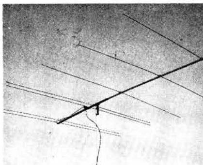
Fig. 4.1: The prototype ZL5-10 five-element 28MHz band ZL Special
