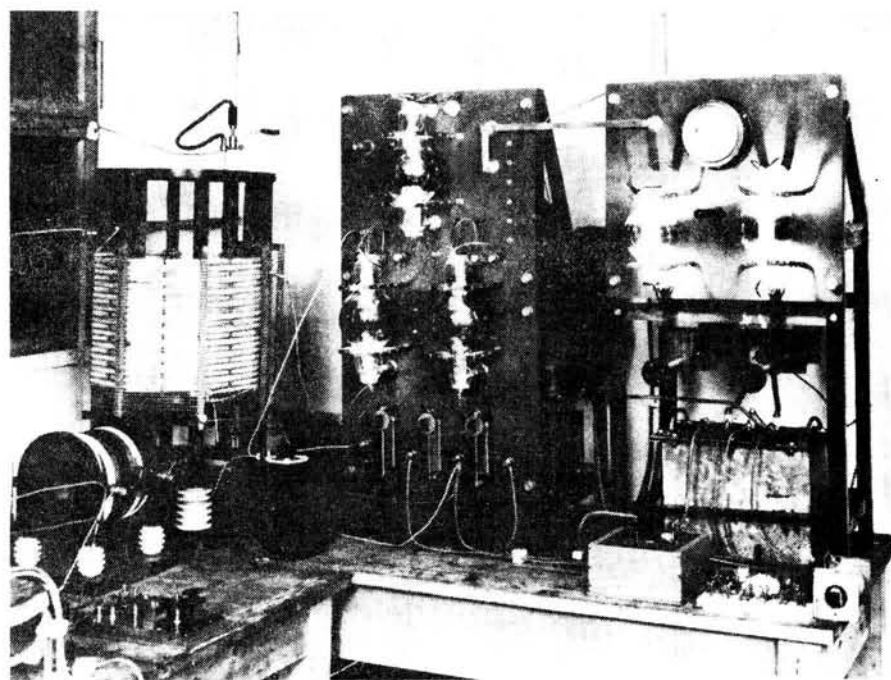
A photograph taken in 1922 of the 2MT Writtle transmitter
