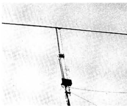
Fig. 4.7: The author's prototype 144MHz Bobtail antenna showing correct mast mounting method
