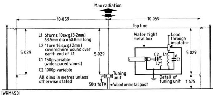
Fig. 4.4: Details of the 14MHz Bobtail antenna
