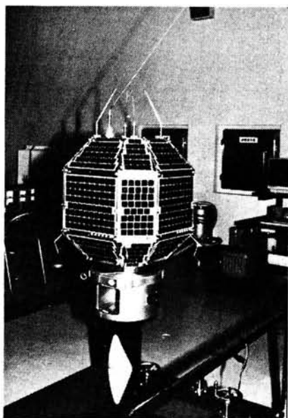
Fig. 5: JAS-1 under test
