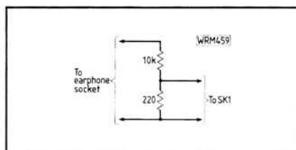
Fig. 6: Signal source attenuator network
