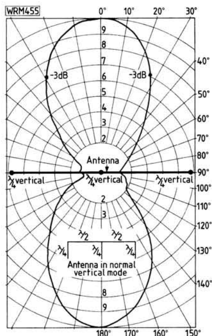
Fig. 4.5: Radiation pattern of the Bobtail broadside antenna
