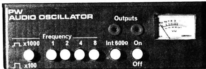
Front panel view of the completed oscillator. Round push-buttons have been used to simplify the cutting of the clearance holes in the panel
