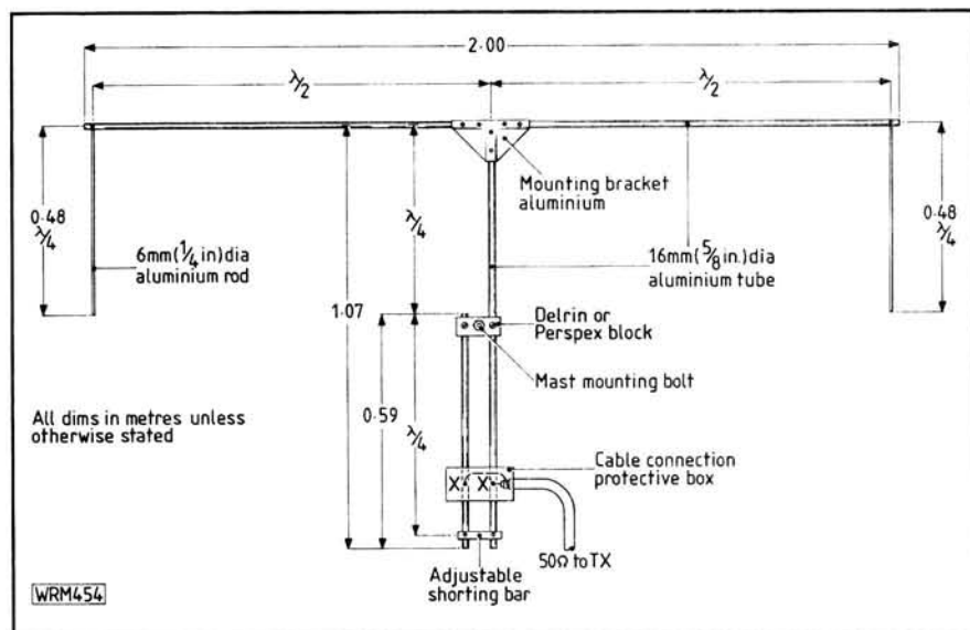
Fig. 4.6: Details of the 144MHz band Bobtail. Bolt to support mast through the stub/feed point insulators
