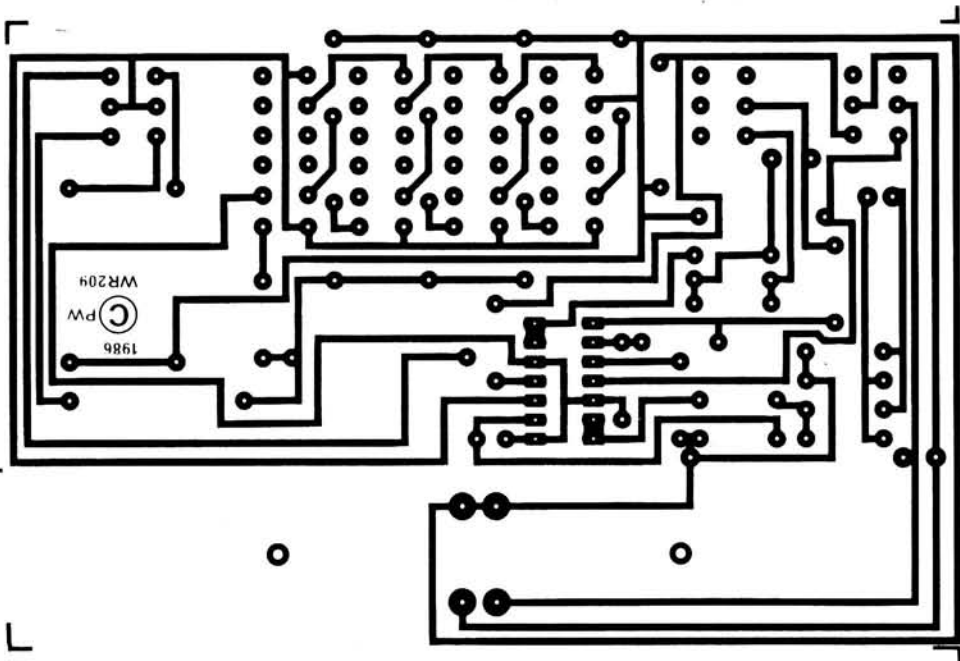
Fig. 2: Full size copper track pattern and component placement drawing for the simple audio oscillator. Although a p.c.b. has been shown here the project could be built using Veroboard or even "ugly" construction. The push-button switches could be replaced by any other type of switch having the required number of poles. The alternative switches would have to be connected using flying leads to the appropriate pads on the p.c.b. The two battery holders are optional—the cheaper flying leads with press stud connectors could be used and in this case the p.c.b. could be cut at the points marked
