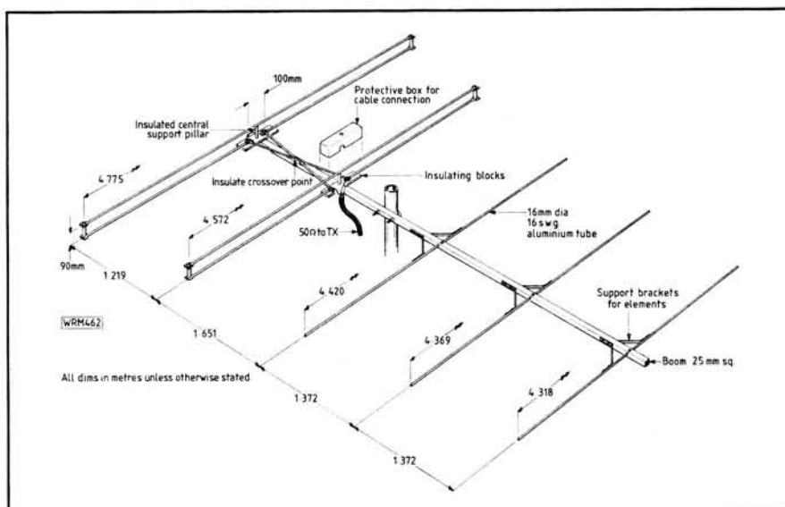
Fig. 4.2: Construction details of the ZL5-10
