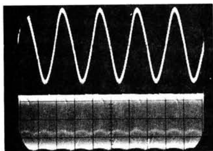
Despite heavy limiting of the r.f. signal (lower trace) the 800Hz sine wave output shows no obvious signs of distortion
